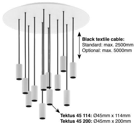
Base Plate (DxH): Ø640 x 37mm
