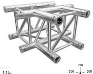
T-STÜCK | JOINT T35 500MM PL CODE F34T35PL
