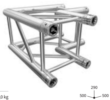
135° ECKE | CORNER C23 CODE F34C23
