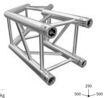
X-STÜCK | JOINT C55 CODE F34C55
