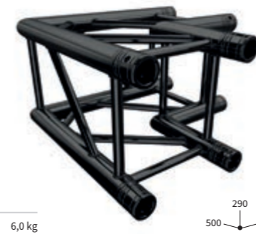
90° ECKE | CORNER C21 CODE F34C21-B
