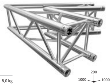
135° ECKE | CORNER C23 PL CODE F34C23PL
