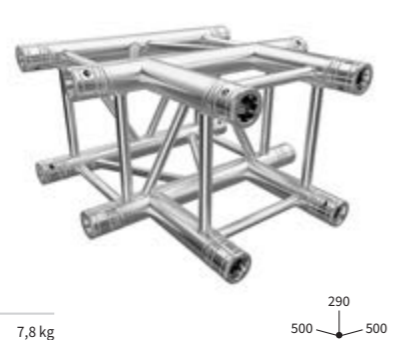
T-STÜCK | JOINT T35 CODE F34T35
