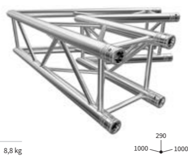
120° ECKE | CORNER C22 CODE F34C22
